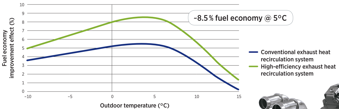
Fuel economy improvement effects of the high-efficiency exhaust heat recirculation system at various outdoor temperatures
