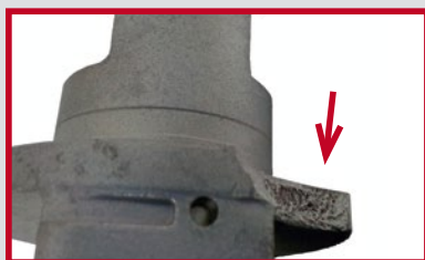
Broken housing/casting
